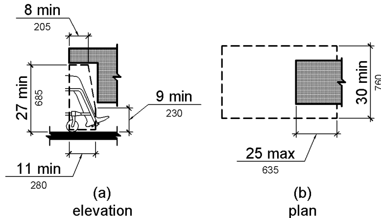
Figure 306.3 Knee Clearance
